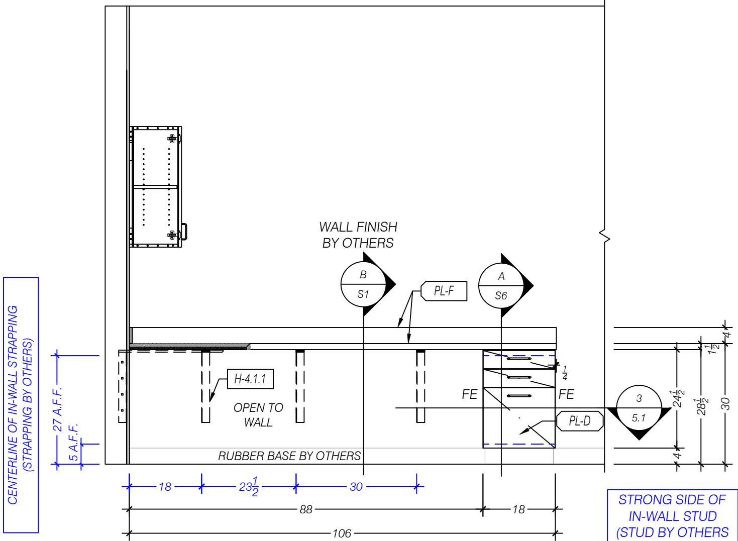
2 ELEVATION SOUTH - MEDIA CONTROL 113 SCALE 1:24 (1/2"=1'-0") ARCH REF: 8/AE408
